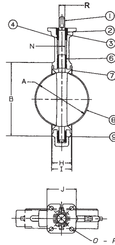
LD-3*22 Lug Style Optional Liner and CF8M Disc
